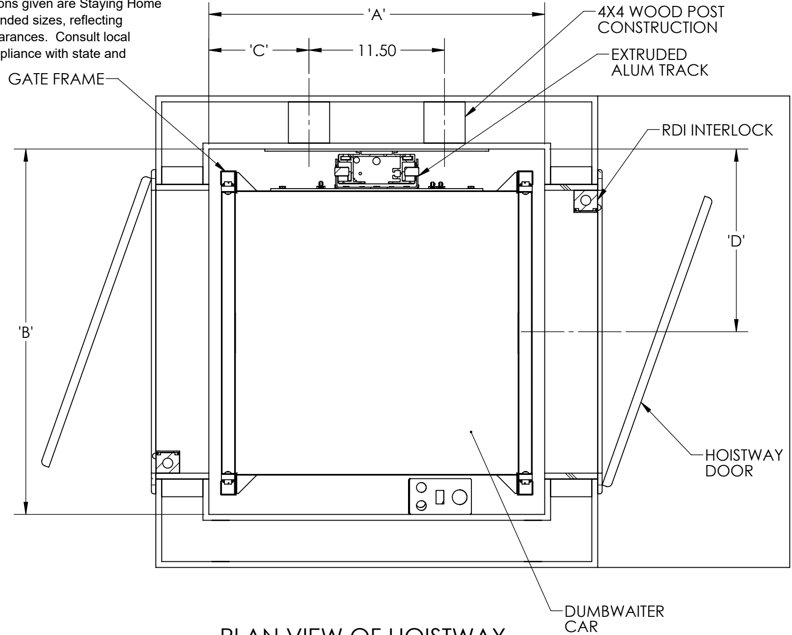
PLAN VIEW OF HOISTWAY
